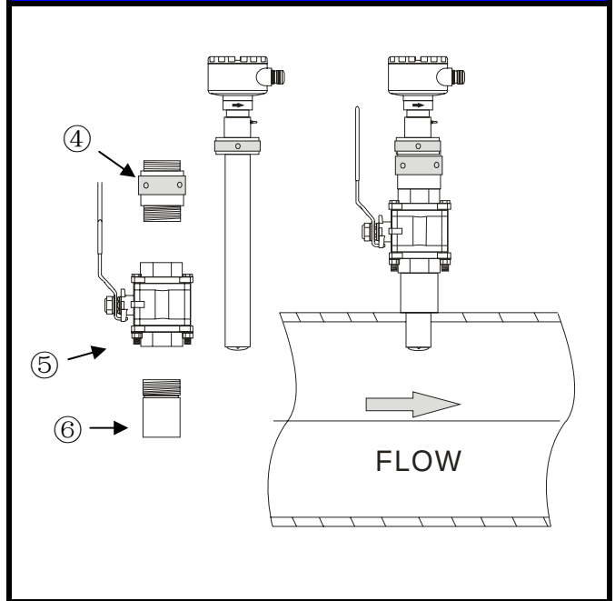
Install with Ball Valve (M60 Thread with Adaptor )
